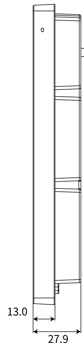
② RIGHT VIEW
